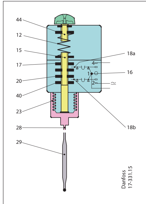
Key sketch RT L temperature control with neutral zone
