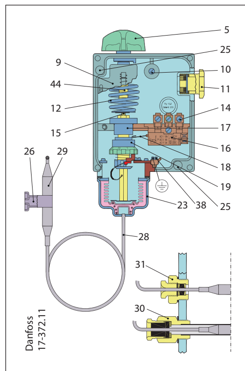
RT temperature control
