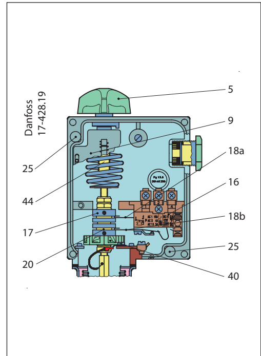
RT L temperature control with neutral zone
