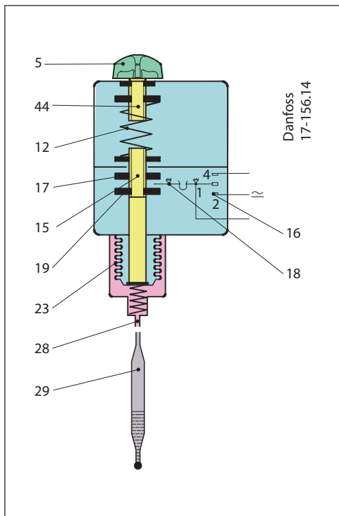
Key sketch of RT temperature control
