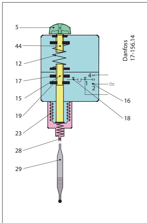
Key sketch of RT temperature control
