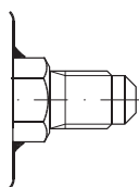
Flare connection
