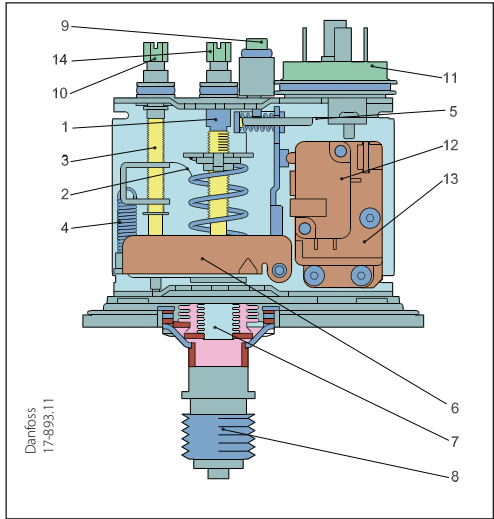
Pressure control, type BCP
