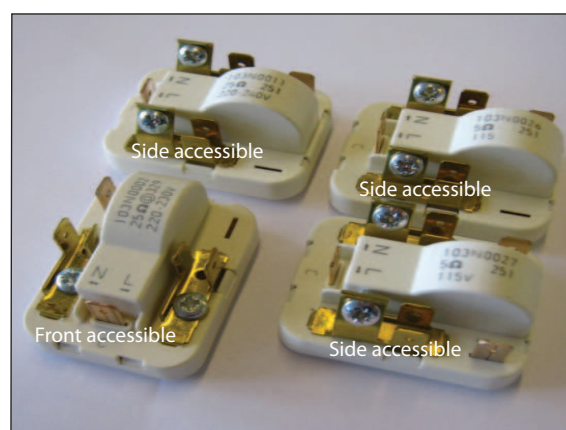
Fig.1 PTC starting devices with front and side accessible screw connections
