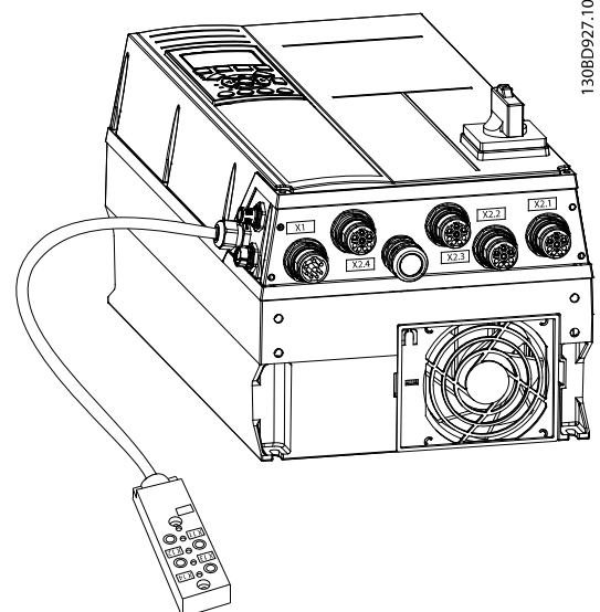
Illustration 3.2 4 Motor Connectors
