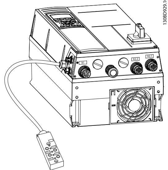
Illustration 3.1 2 Motor Connectors
