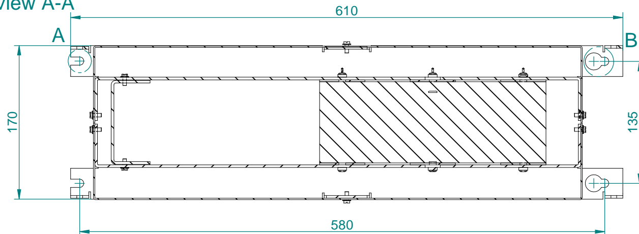
sectional view A-A
