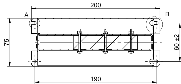
sectional view C-C
