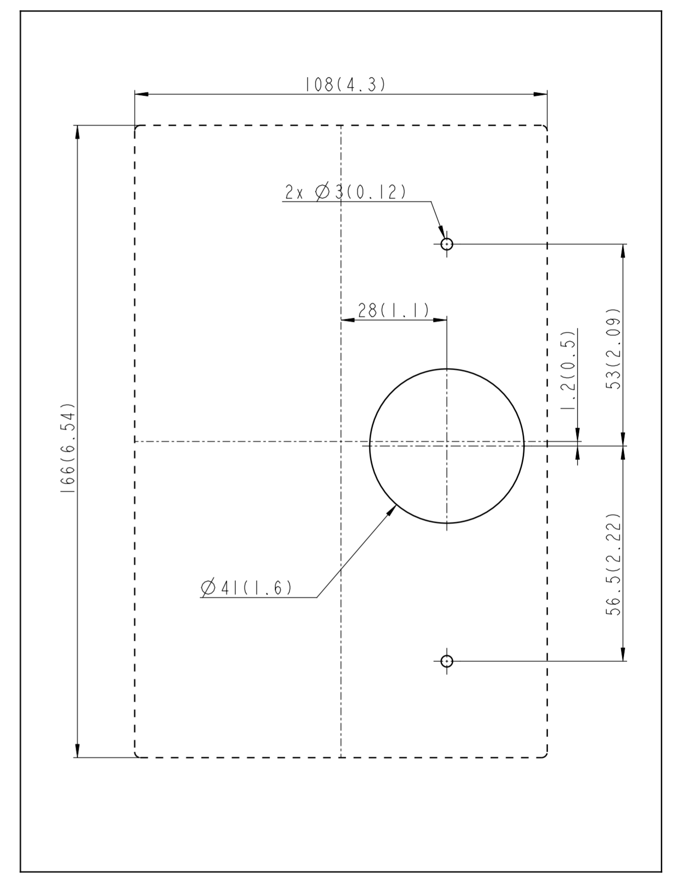
Surface Mounting Drilling Template View from front in mm(in)
