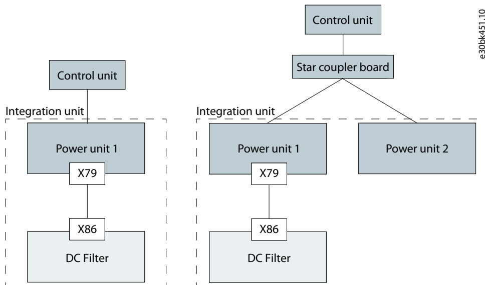
Illustration 14: AuxBus Topology
