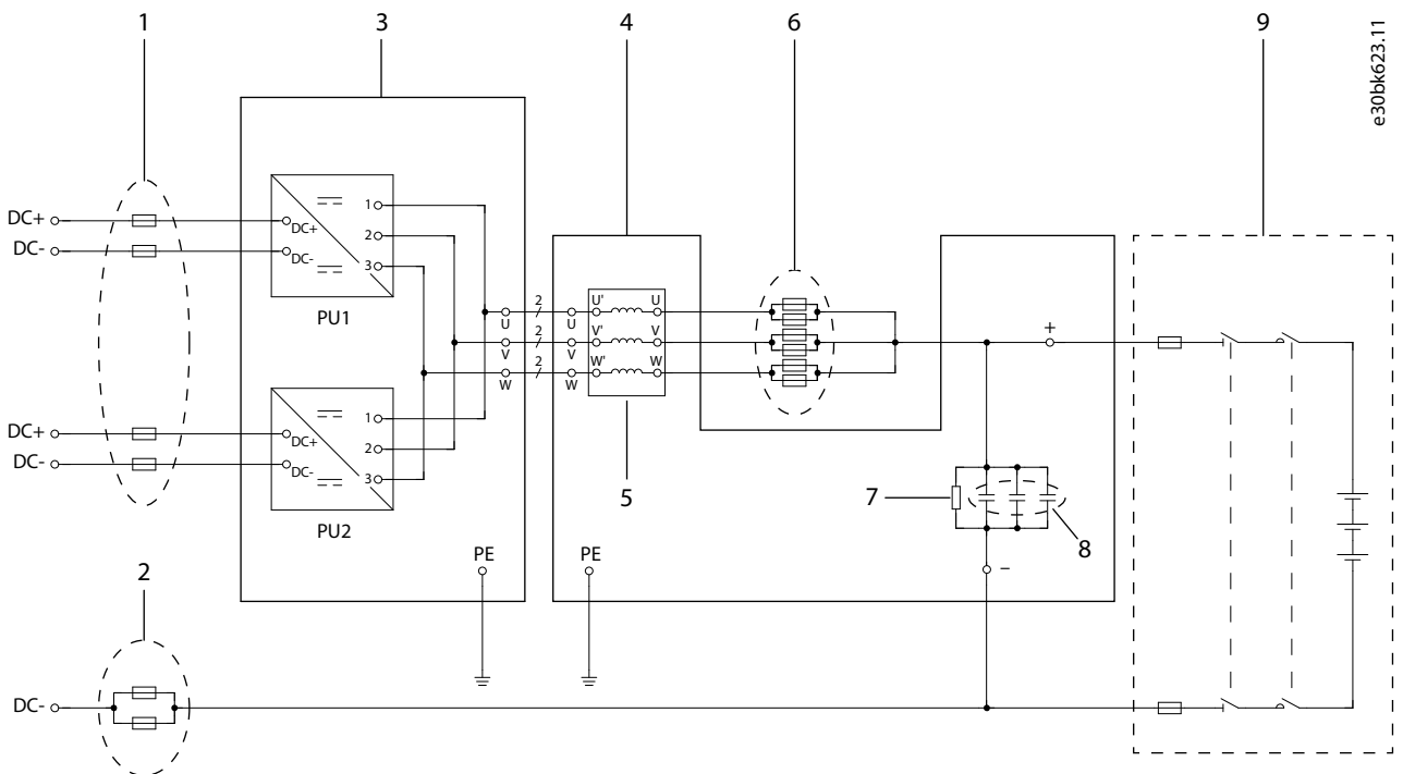
Illustration 17: Wiring Diagram, DC12L
