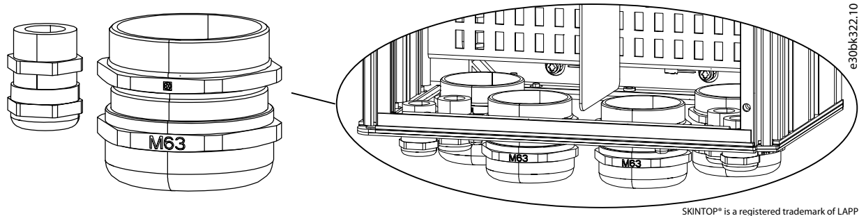
Illustration 6: Cable Entry Plate with SKINTOP® Cable Glands
