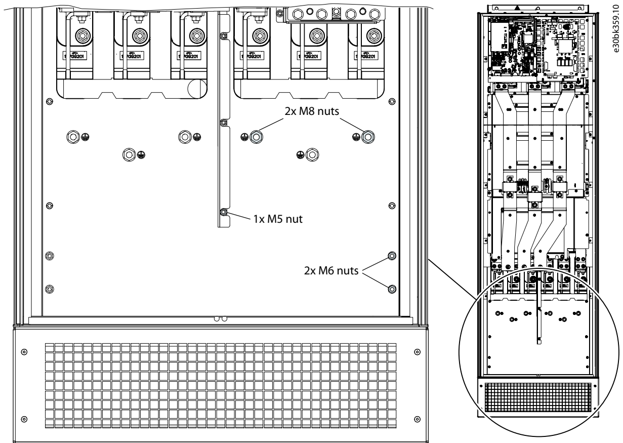
Illustration 4: Existing Fasteners to Use for Filter Installation
