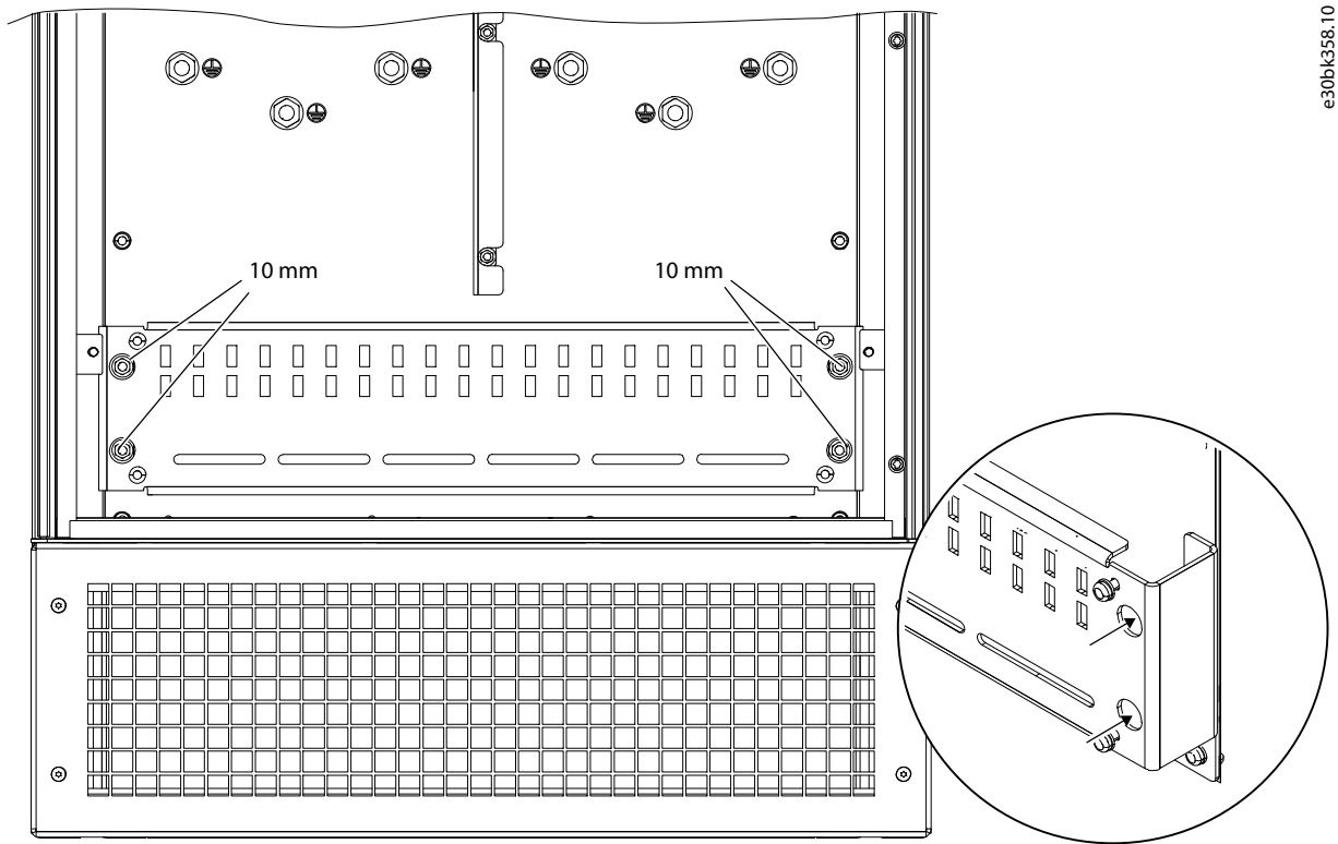
Illustration 3: Inner Cable Bracket Removal
