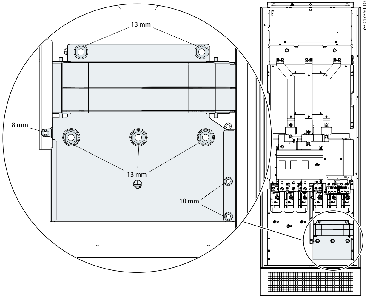
Illustration 5: Common-mode Filter Installation
