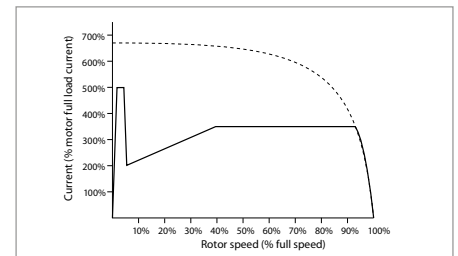
Constant current/ current ramp – here shown with kickstart
