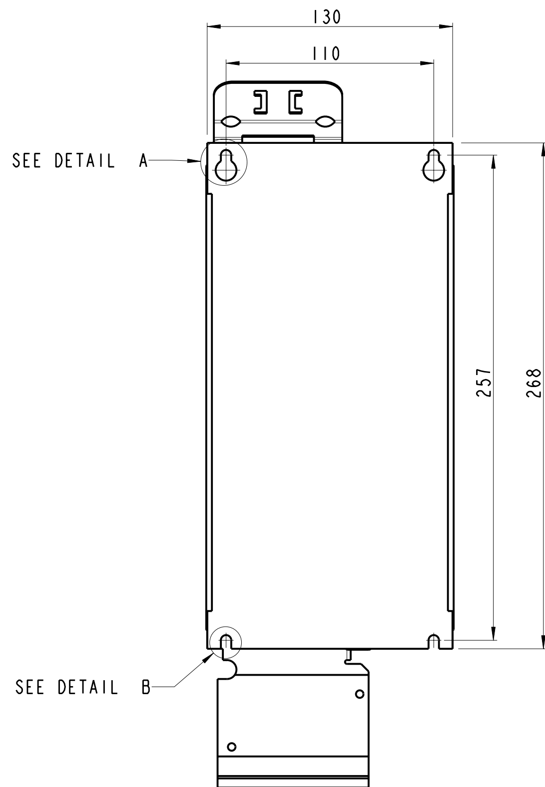
MOUNTING BASE
