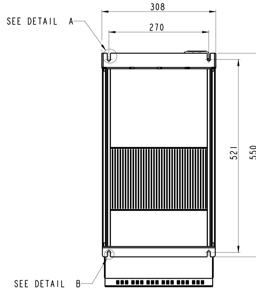
MOUNTING BASE
