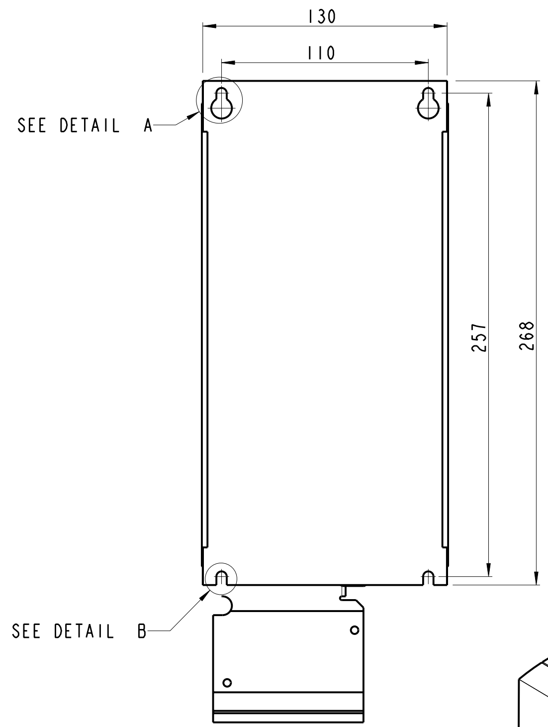
MOUNTING BASE
