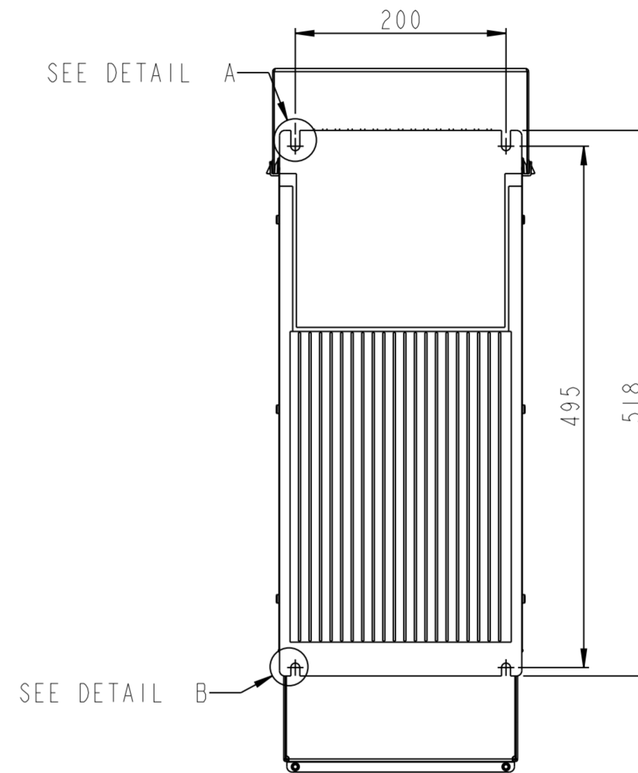
MOUNTING BASE
