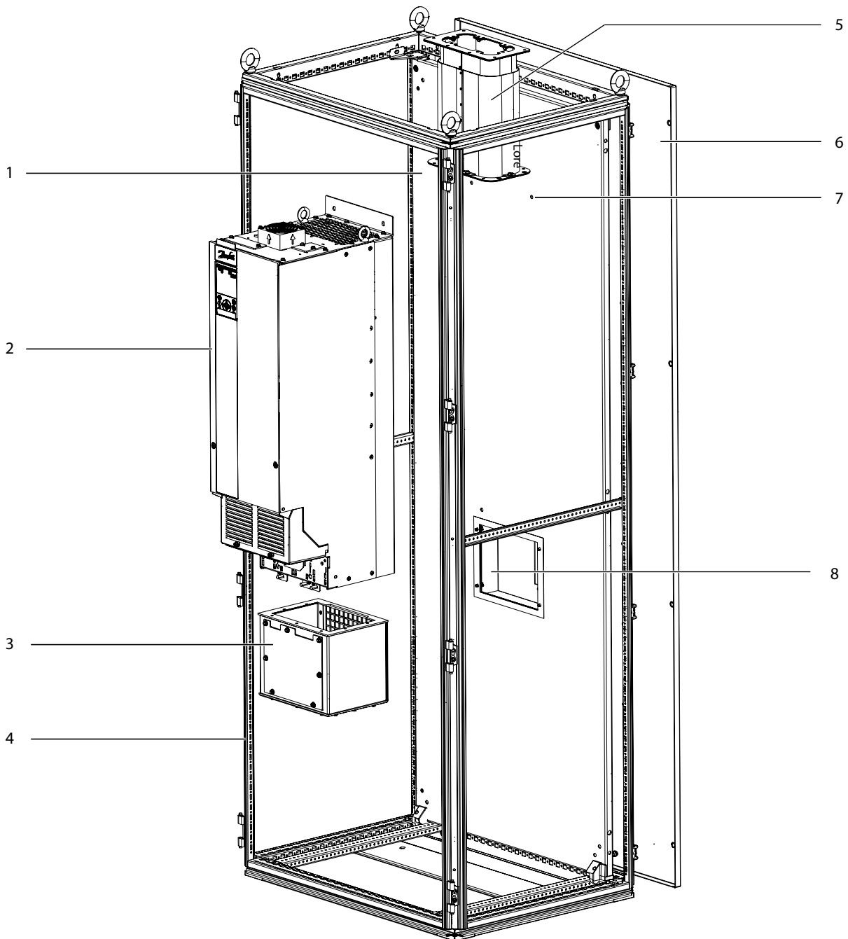
Illustration 2: Overview of In-back/Out-top; Cooling Kit
