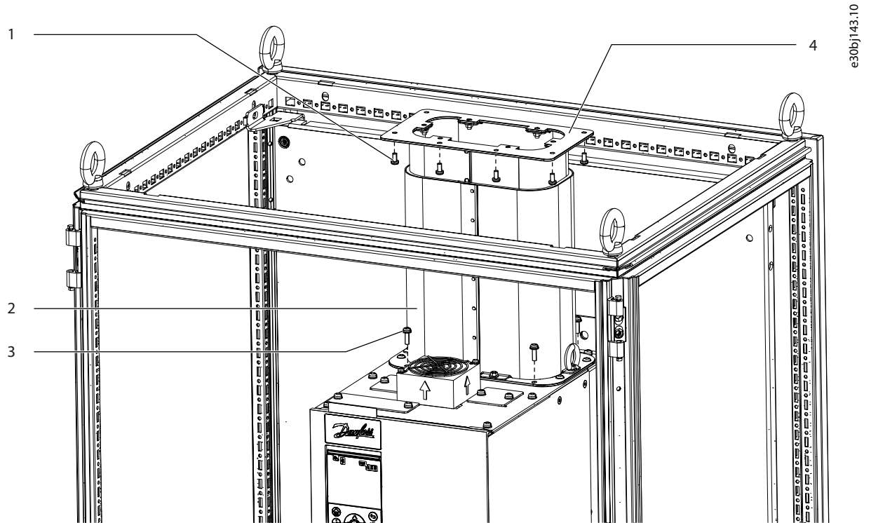
Illustration 11: Installation of the Top Duct
