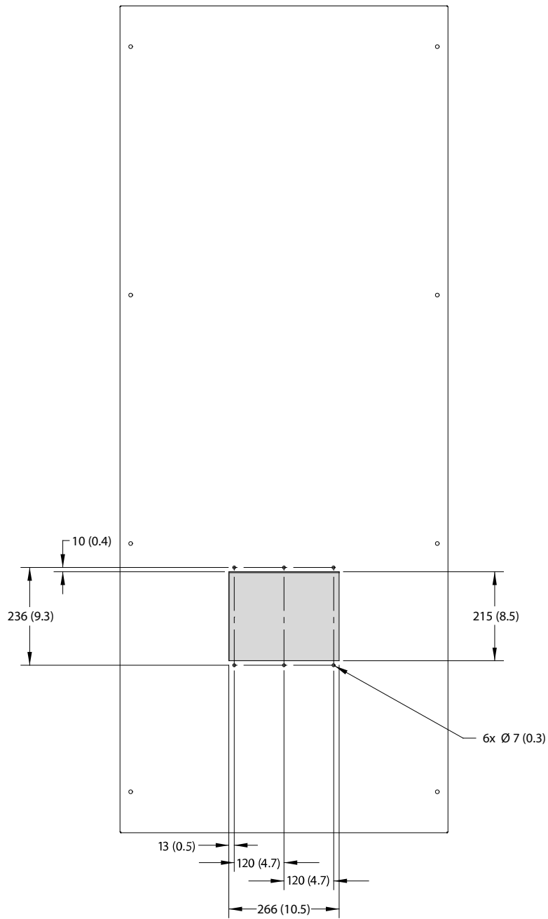
Illustration 7: FA09 Cabinet Back Plate Template for In-back/Out-top Cooling
