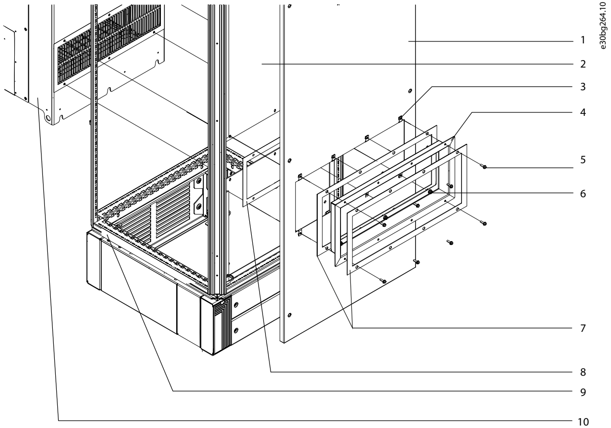
Illustration 12: Installation of the Frequency converter, Mounting Plate, Backplate, and Back Duct
