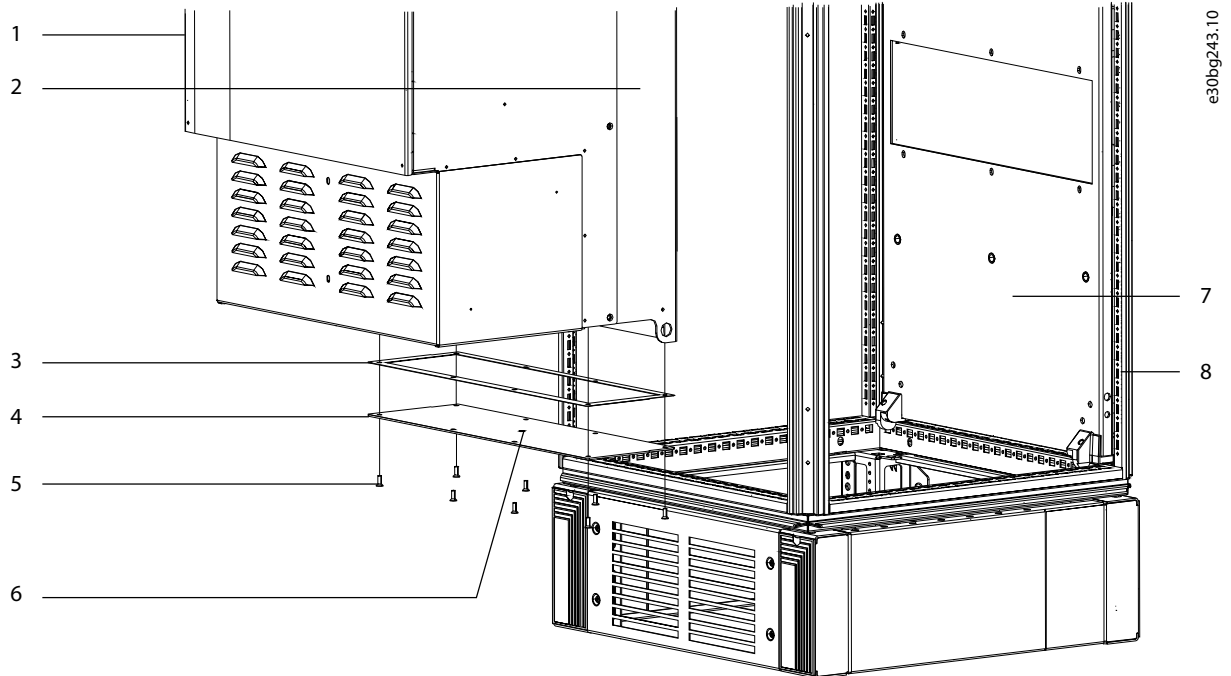
Illustration 11: Installation of the Bottom Cover
