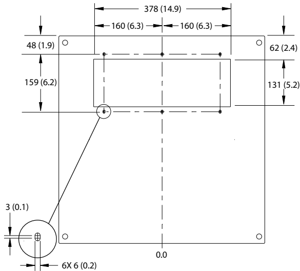
Illustration 8: Dimensions for Opening in Cabinet Top Plate
