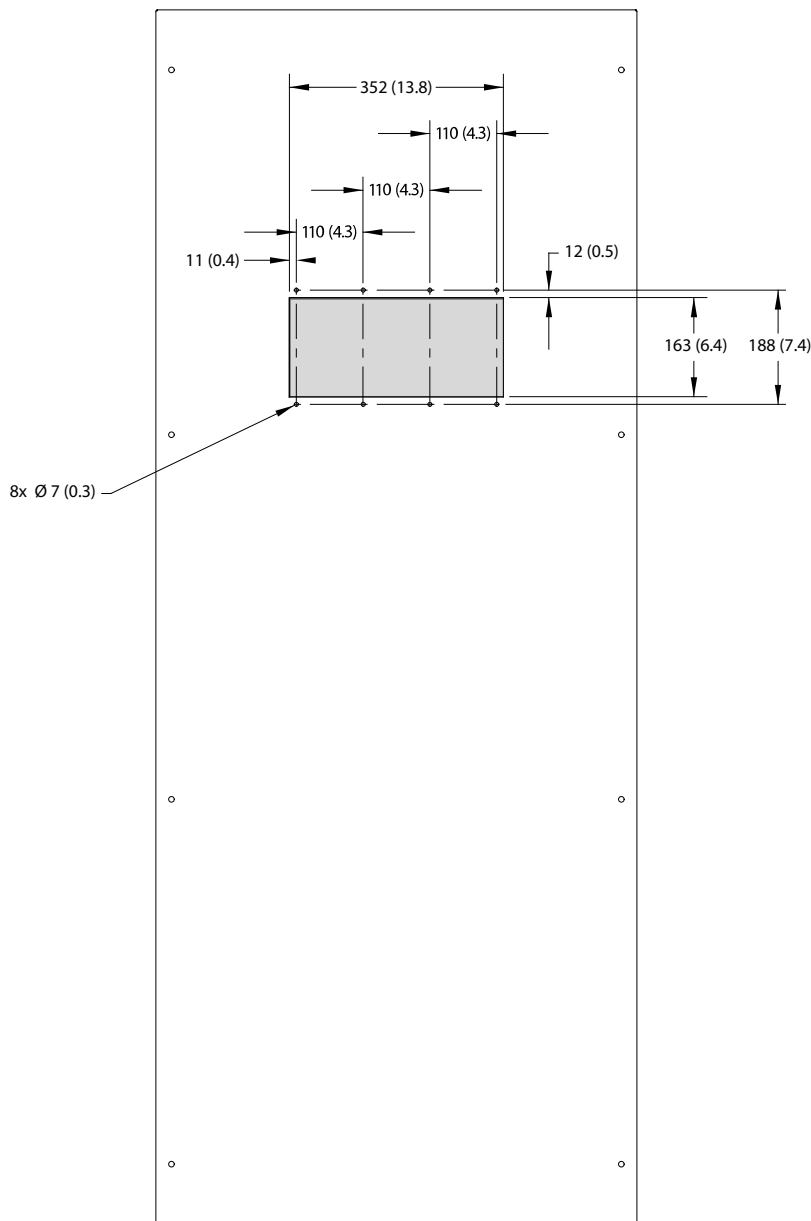
Illustration 6: FA10 Cabinet Backplate Template for In-bottom/Out-back Cooling
