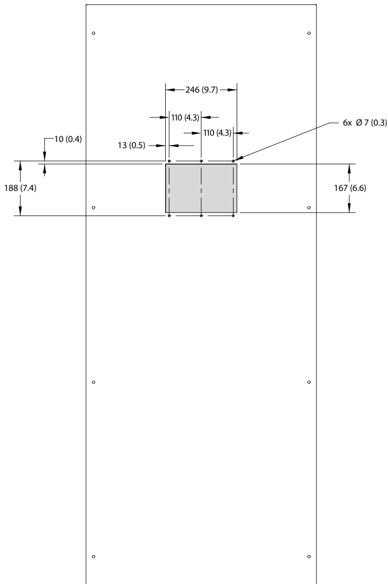
Illustration 5: FA09 Cabinet Backplate Template for In-bottom/Out-back Cooling
