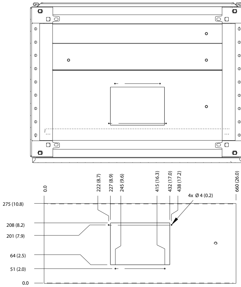
Illustration 8: FA09 Base Plate Template
