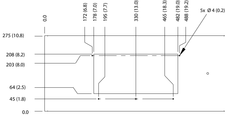
Illustration 9: FA10 Base Plate Template
