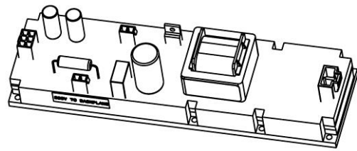
Figure 2 – Potted DC-DC Converter
