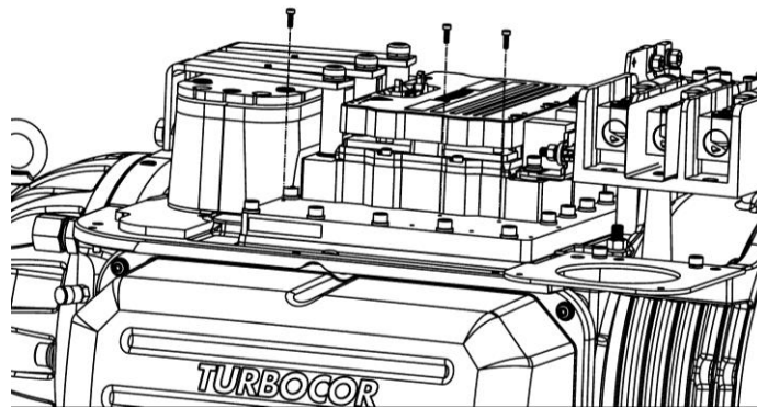
Figure 9 – Rear Open Frame DC-DC Fasteners
