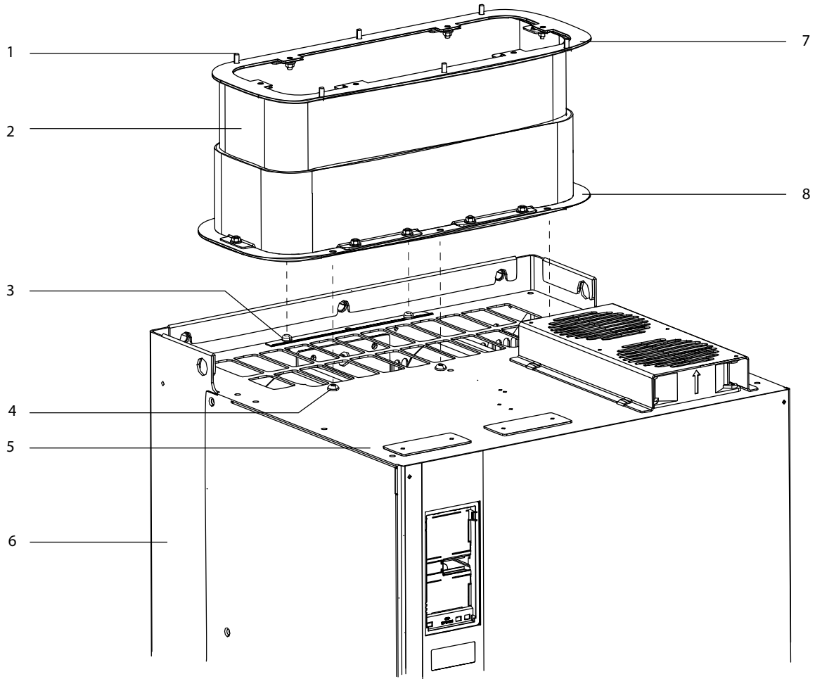
Illustration 8: Installation of the Top Duct Over the Top Vent
