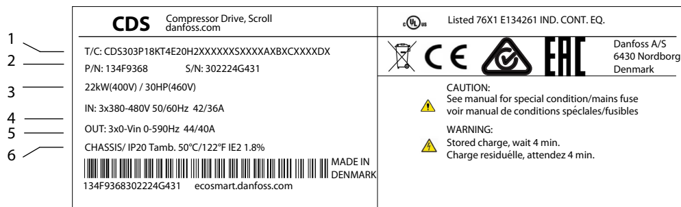
Illustration 1: Example of the Type Code on the Product Label
