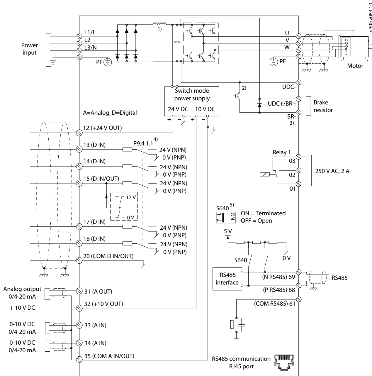
Illustration 28: Wiring Diagram
