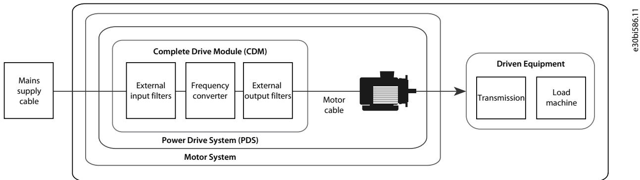
Illustration 3: Drive System Design
