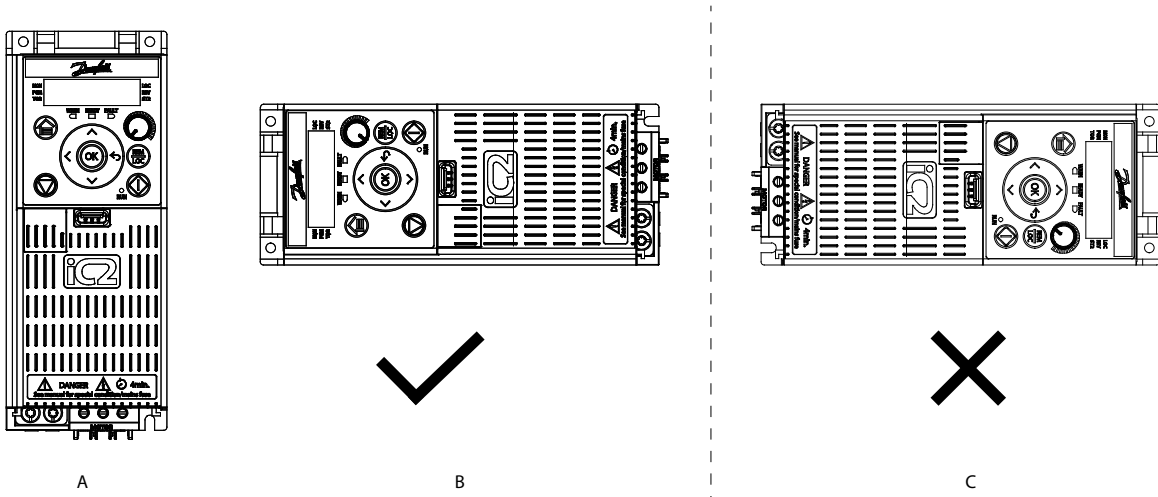
Illustration 24: Mounting Directions for Drives
