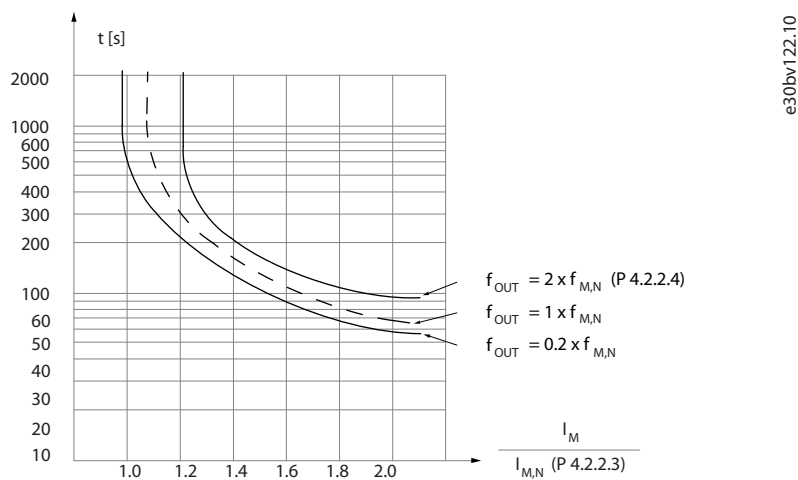
Illustration 36: ETR
