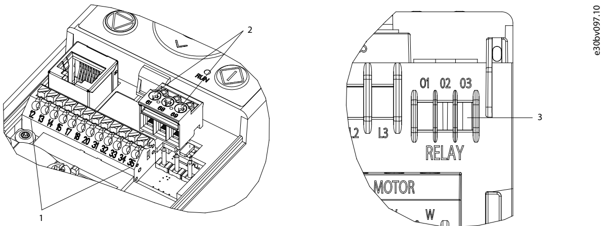
Illustration 40: Control Terminal Numbers and Locations
