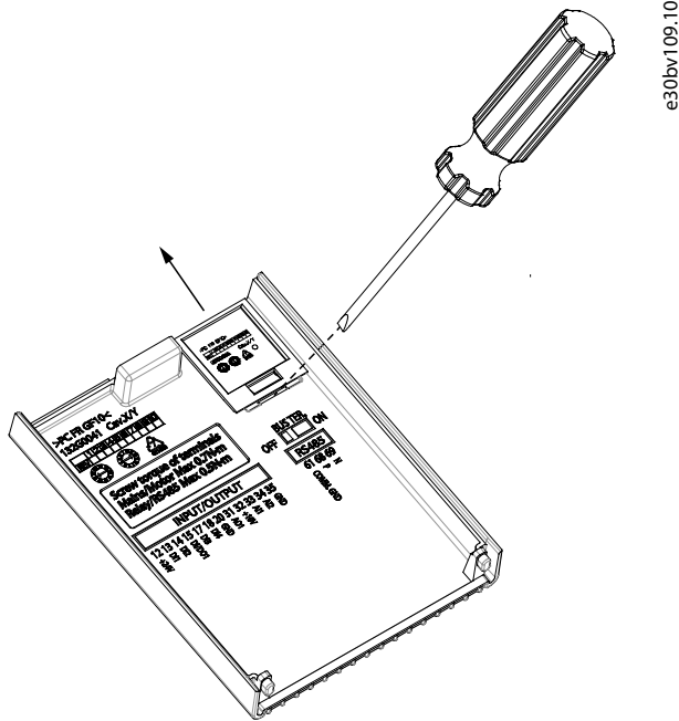
Illustration 10: Removing the Sliding Door
