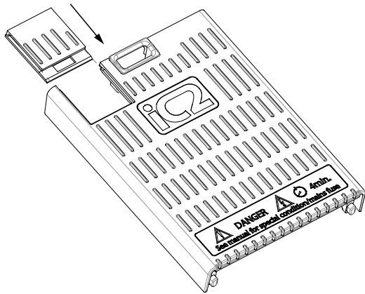
Illustration 11: Installing the Sliding Door
