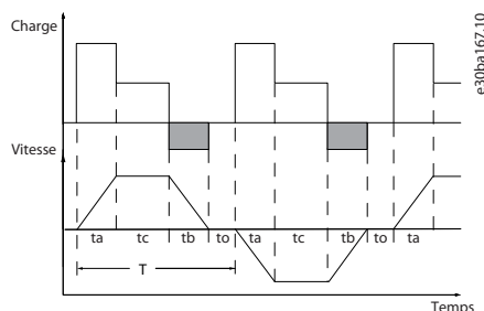
Illustration 12: Cycle de freinage type
