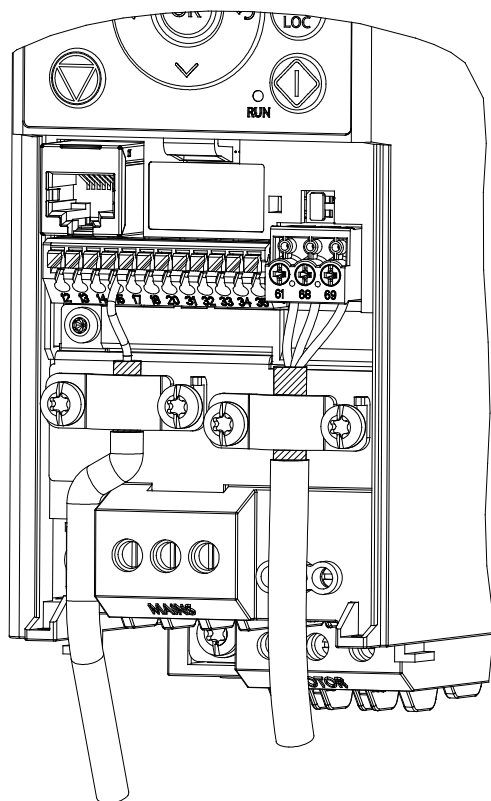
Illustration 42: Raccordement correct du blindage de câble
