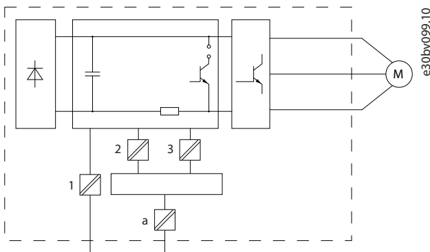
Illustration 36: Isolation galvanique
