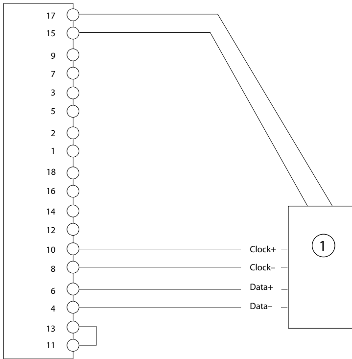
Illustration 16: Wiring Configuration for 2-Track EnDat Encoder
