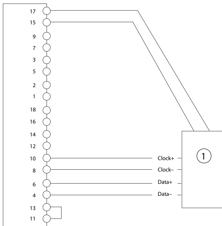
Illustration 13: Wiring Configuration for 2-Track SSI Encoder
