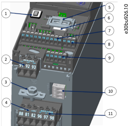
Illustration 35: Terminal Numbers
