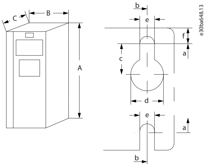
Illustration 19: Top and Bottom Mounting Holes
