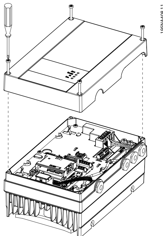
Illustration 4.7 Fjern frontpanelet
