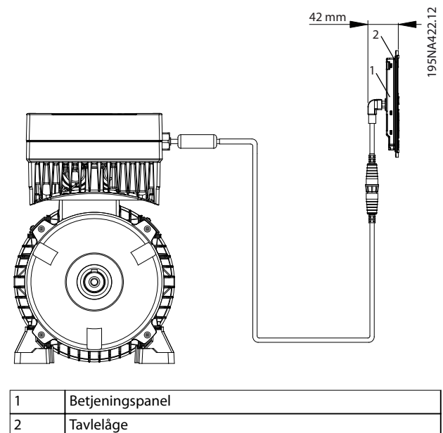
Illustration 5.3 LCP-frembygning
