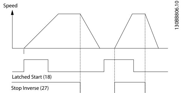
Illustration 8.2 Pulsstart/inverteret stop
