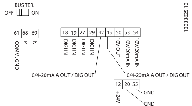
Illustration 1.25 Control Terminals
