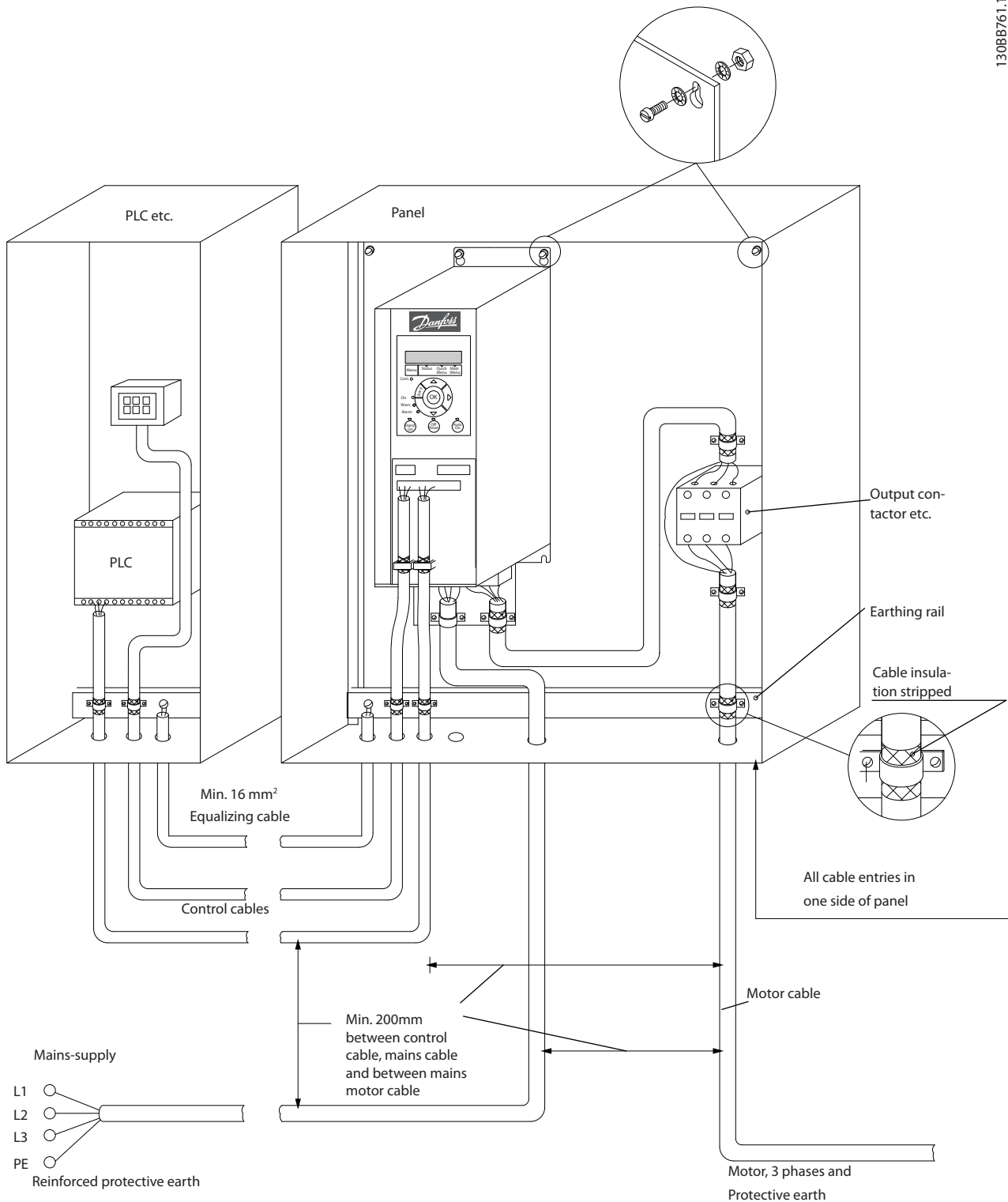
Illustration 1.21 EMC-correct Electrical Installation
