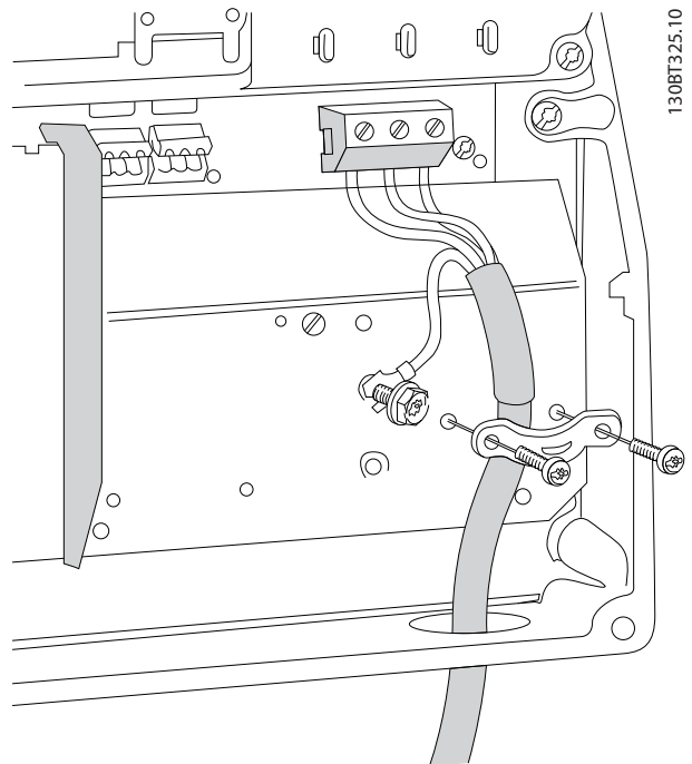
Illustration 1.18 I6 Frame IP54 380-480 V 22-37 kW
