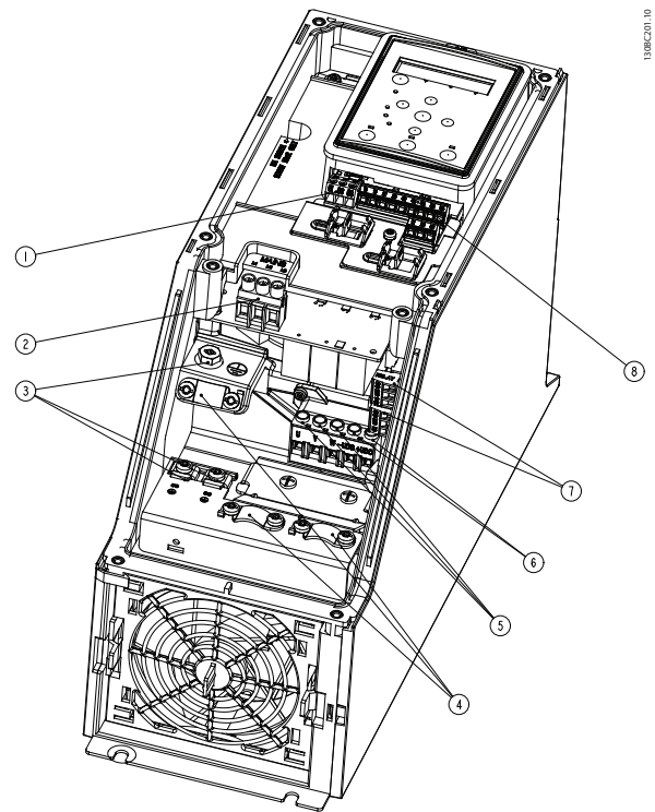
Illustration 1.14 I3 Frame IP54 380-480 V 5.5-7.5 kW
