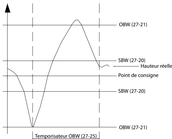
Illustration 3.78 Tps OBW
