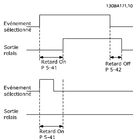
Illustration 3.25 Relais, retard ON
