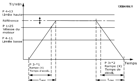
Illustration 3.17 Rampe 1
