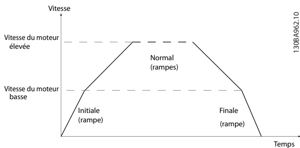
Illustration 3.19 Tps rampe initial et final
