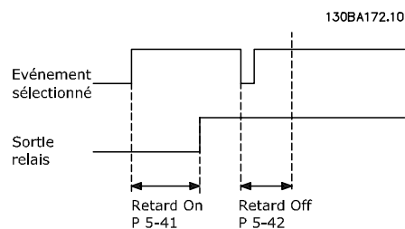
Illustration 3.26 Relais, retard OFF
