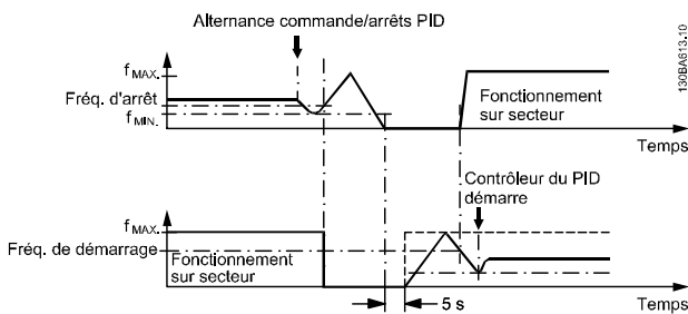
Illustration 3.85 Configuration lente
