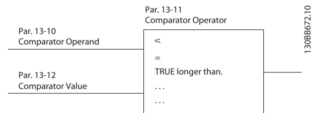
Illustration 3.37 Compareurs
