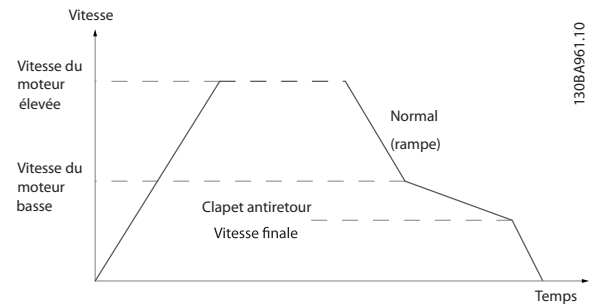
Illustration 3.20 Rampe clapet anti-retour
