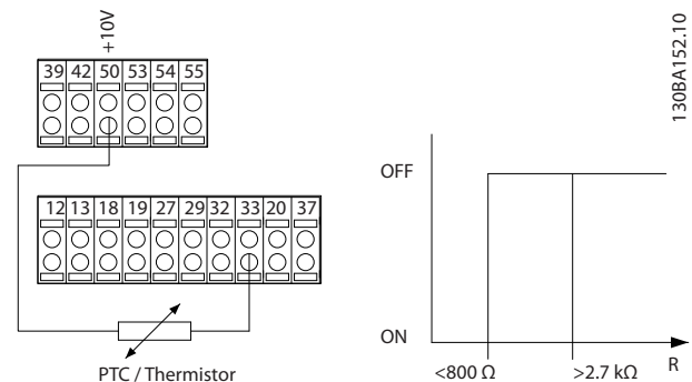
130BA152.10 Ilustrasi 3.13 Sambungan Termistor PTC - Input Digital
