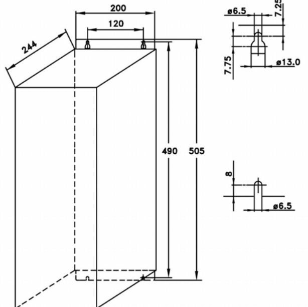
VLT 2880-2882 380-480V
