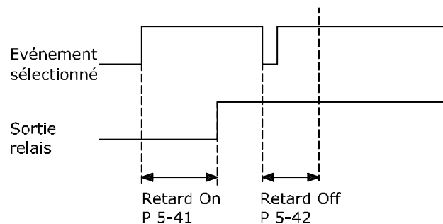
Illustration 3.37 Relais, retard OFF
