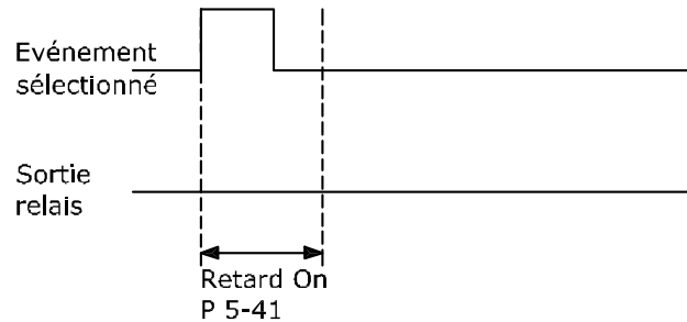
Illustration 3.36 Relais, retard ON
