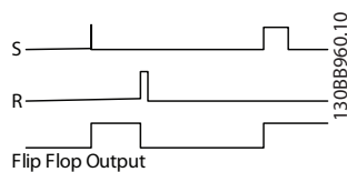
Illustration 3.55 Sorties bascules
