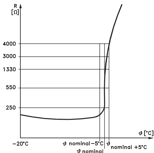
175HA183.10 Illustration 6.2 Perfil do PTC
