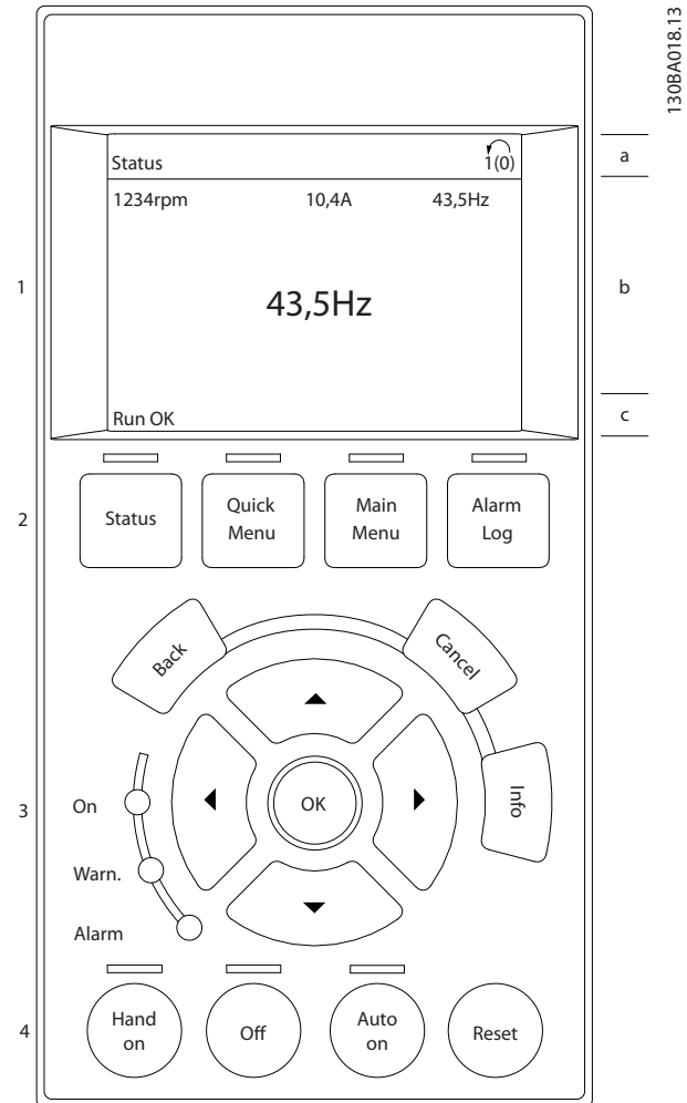
Illustration 5.1 LCP
