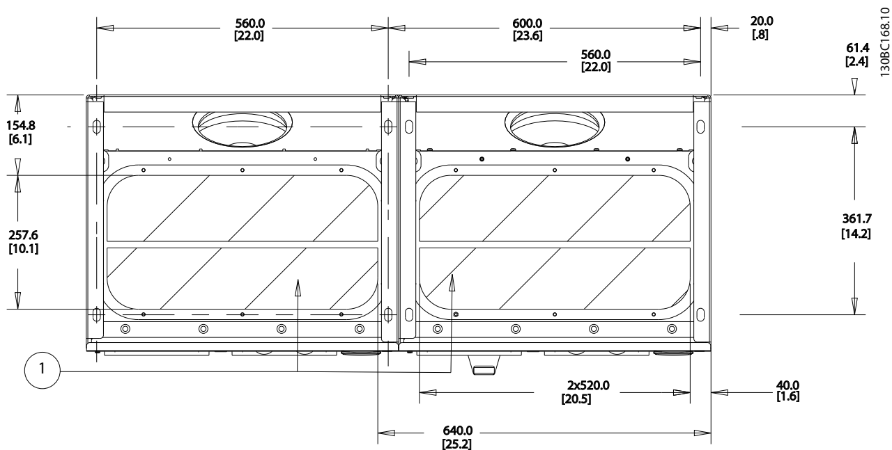
Illustration 4.20 Chassi de Tamanho E9
