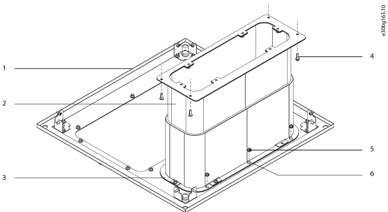
Illustration 1.7 Installation of the Bottom Duct on the Base Plate
