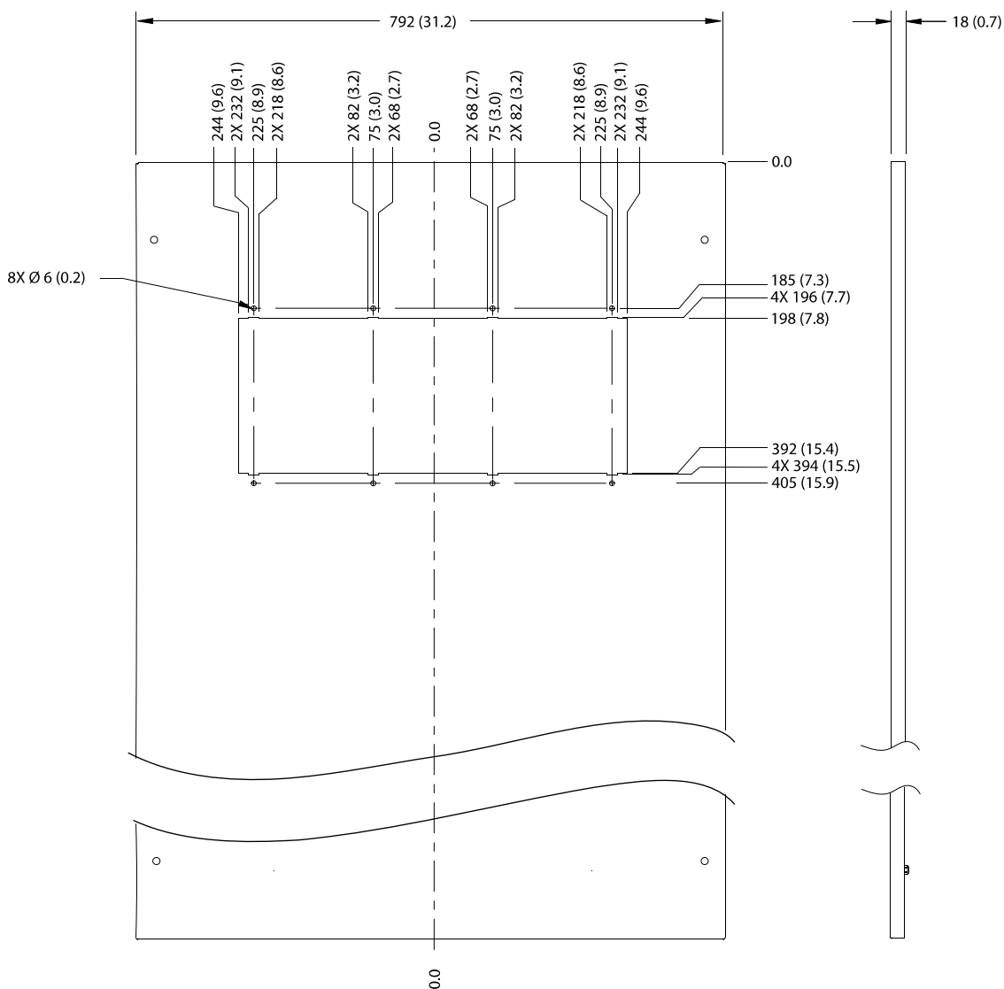
Illustration 1.4 Vent Dimensions for Backplate in 800 mm (32 in) Enclosure
