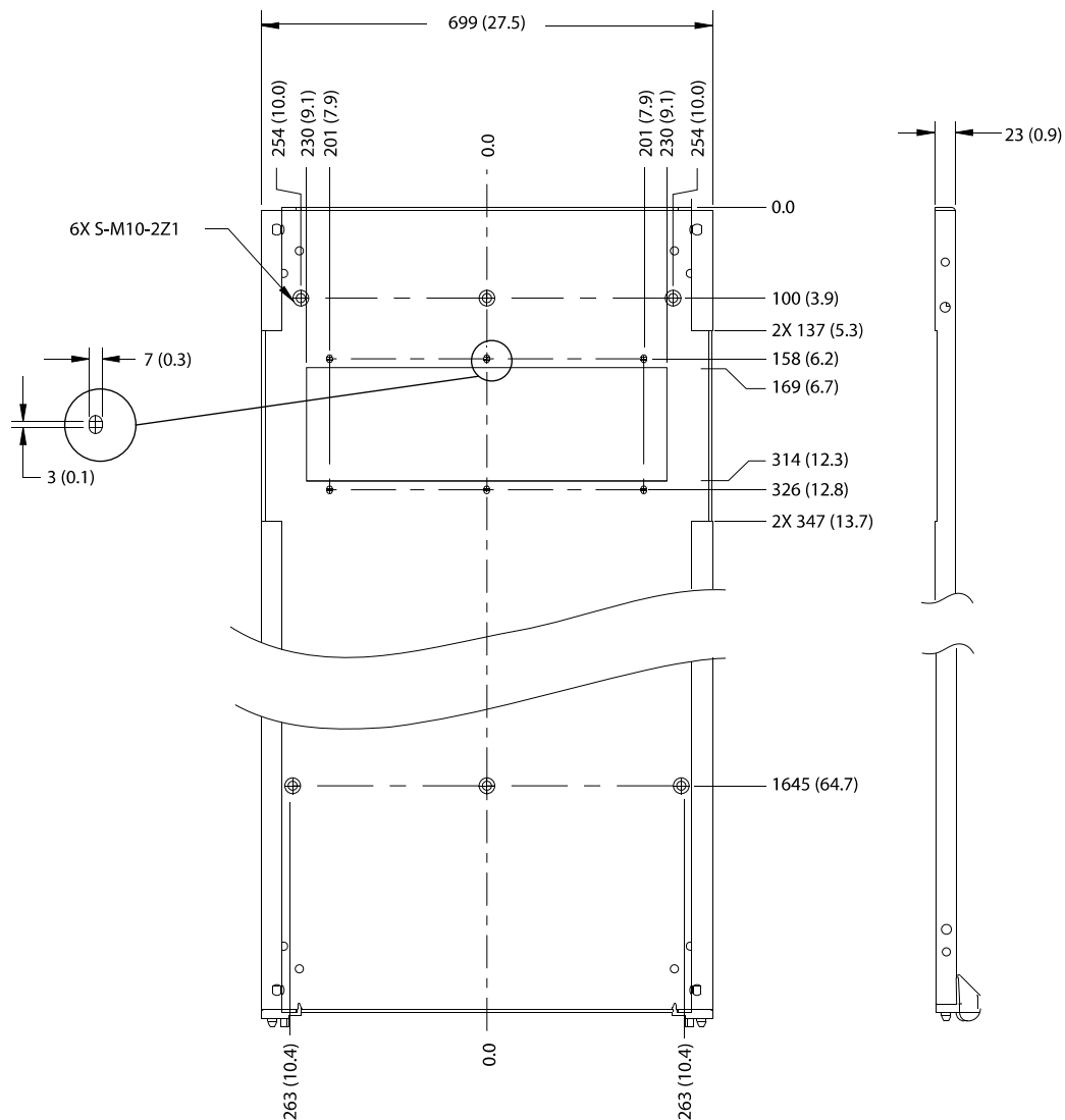
Illustration 1.3 Vent Dimensions for Mounting Plate in 800 mm (32 in) Enclosure
