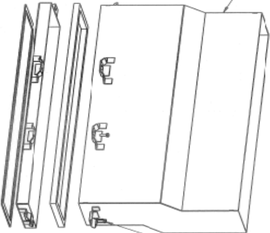
4 X M5 X 16MM TORX SCREW
