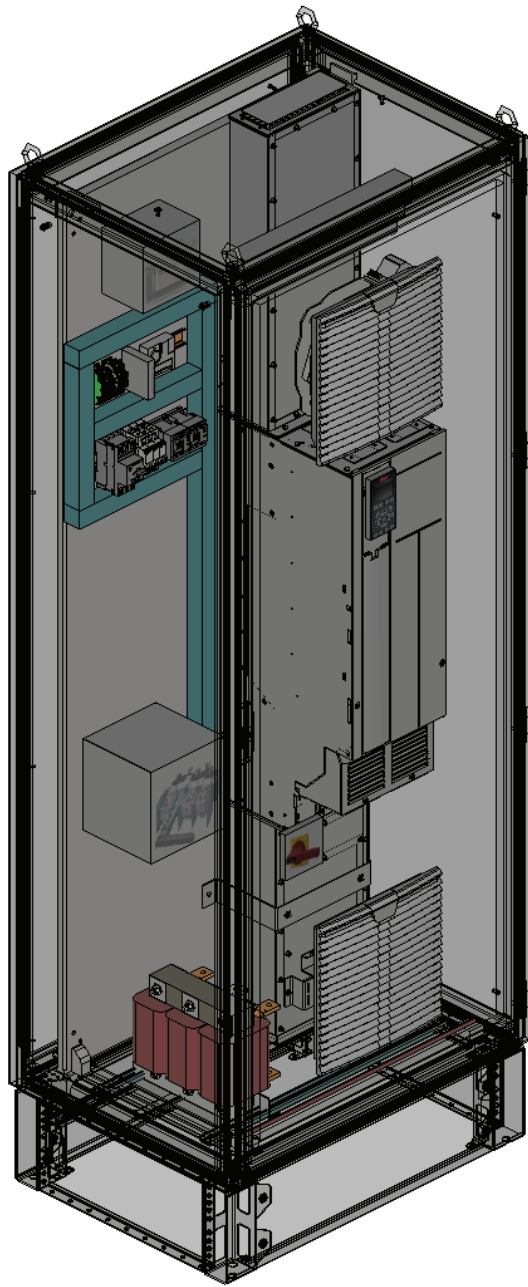
3D mounting layout 3D-Montageaufbau
