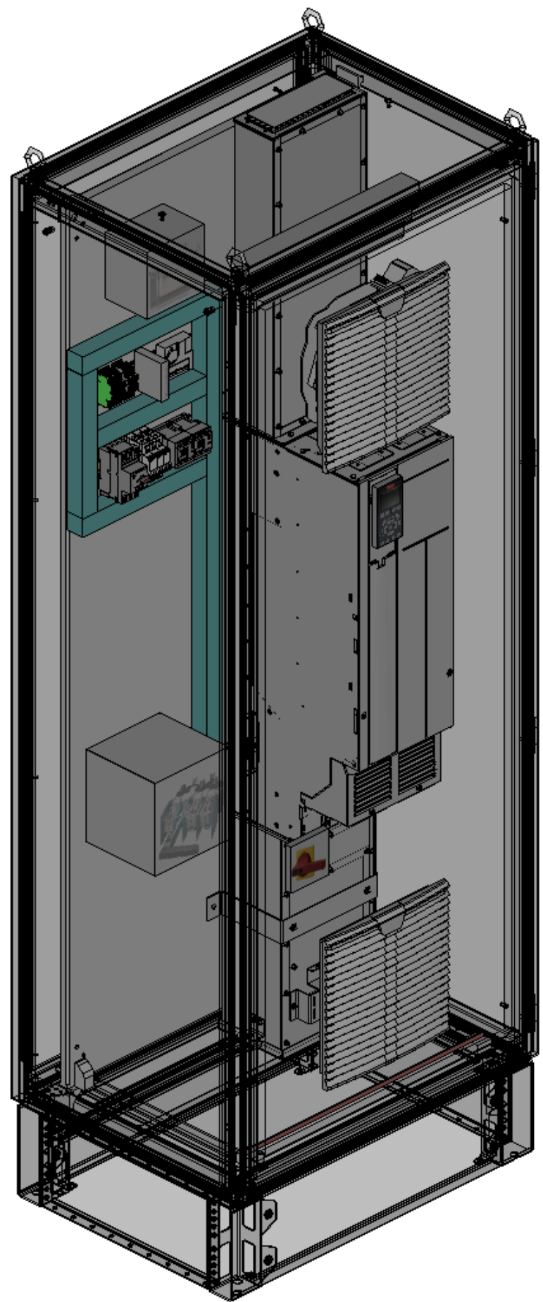
3D mounting layout 3D-Montageaufbau
