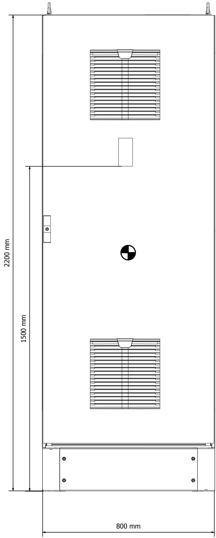
Front view Frontansicht
