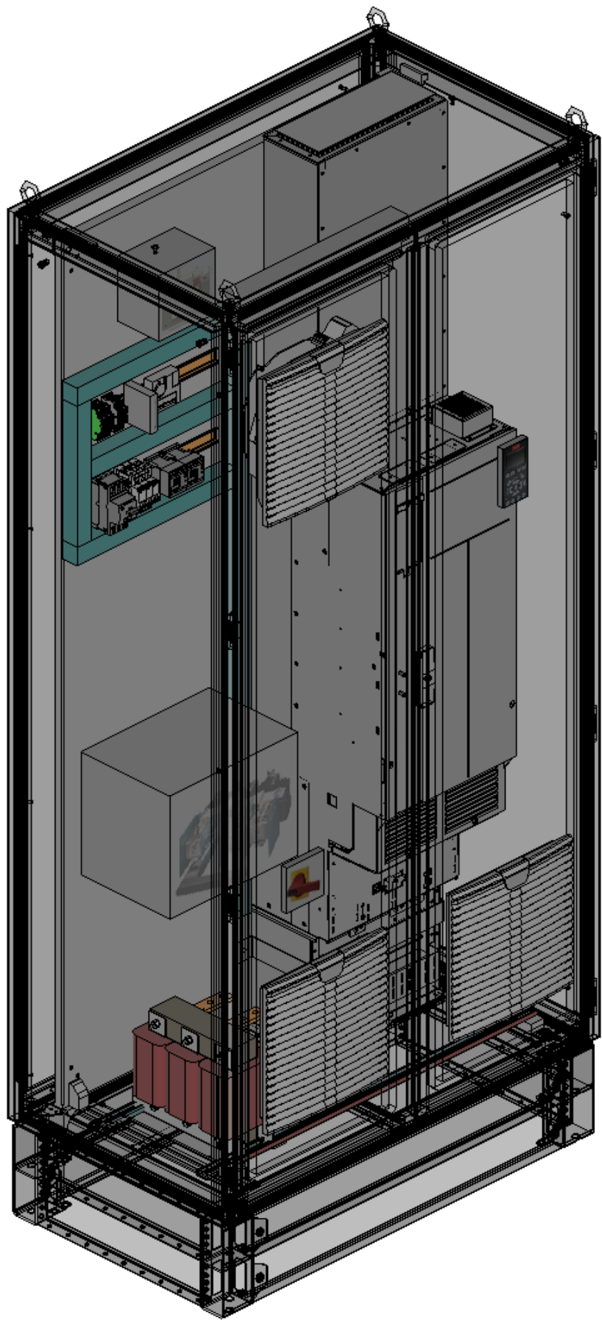
3D mounting layout 3D-Montageaufbau
