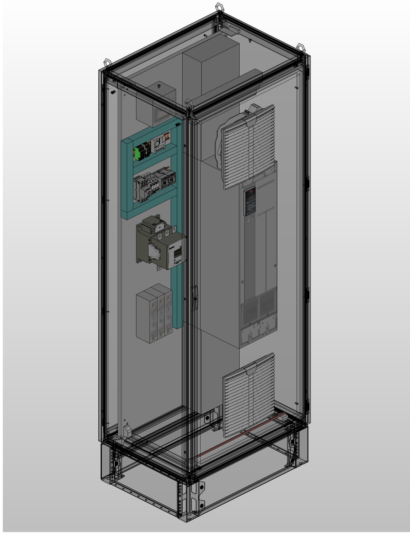
3D mounting layout 3D-Montageaufbau
