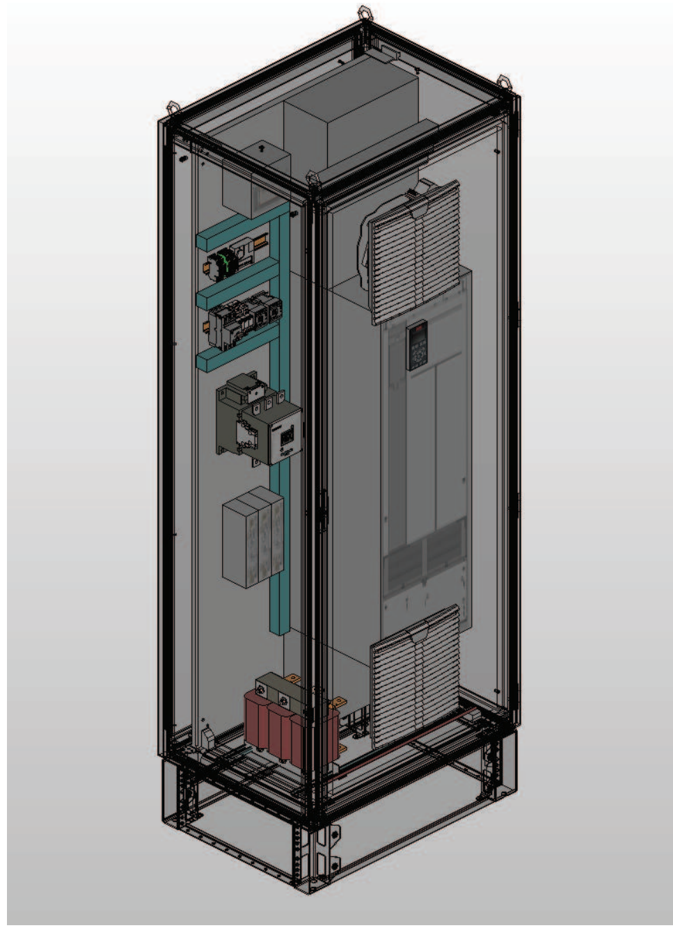
3D mounting layout 3D-Montageaufbau
