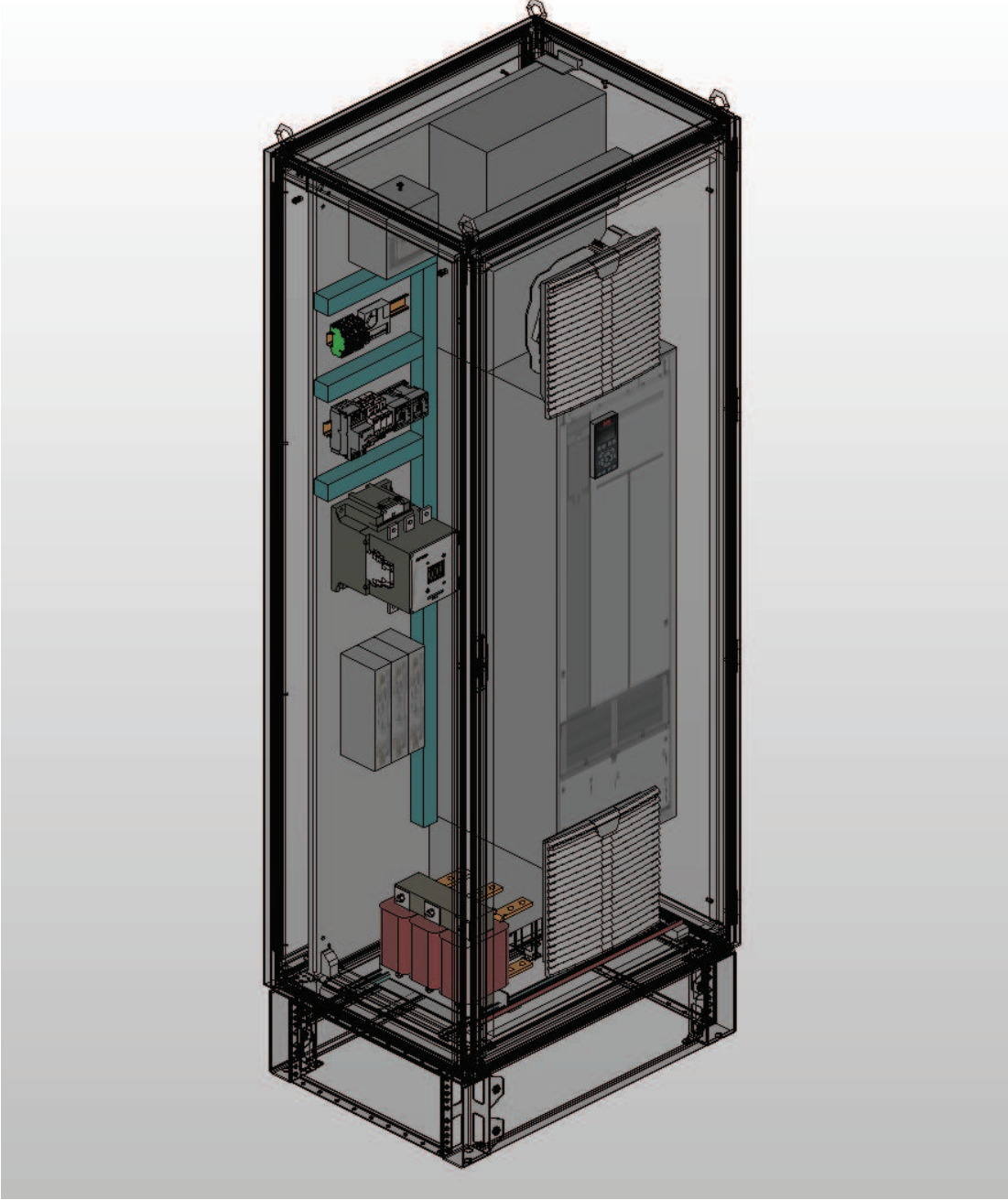
3D mounting layout 3D-Montageaufbau
