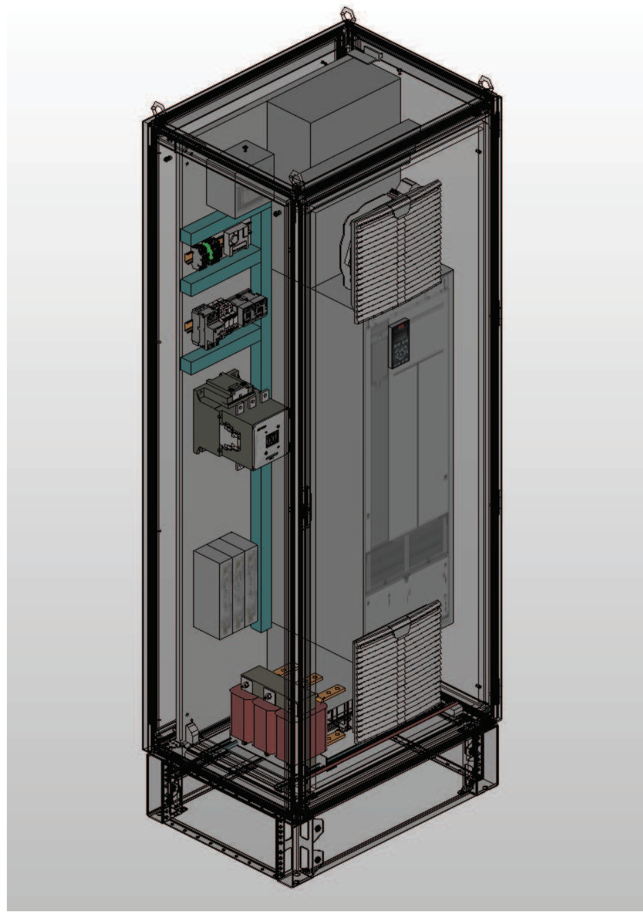
3D mounting layout 3D-Montageaufbau
