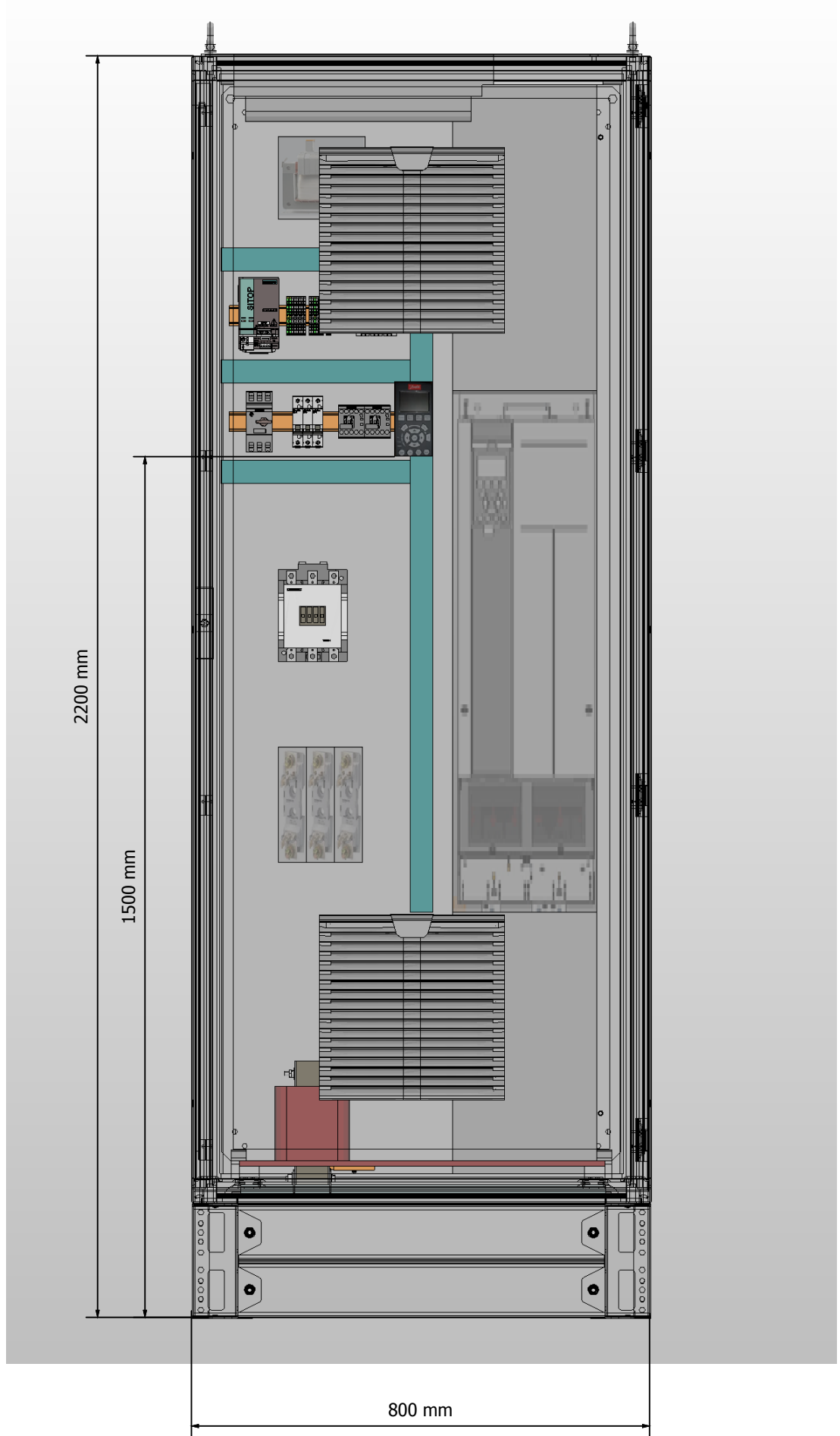
Front view Frontansicht
