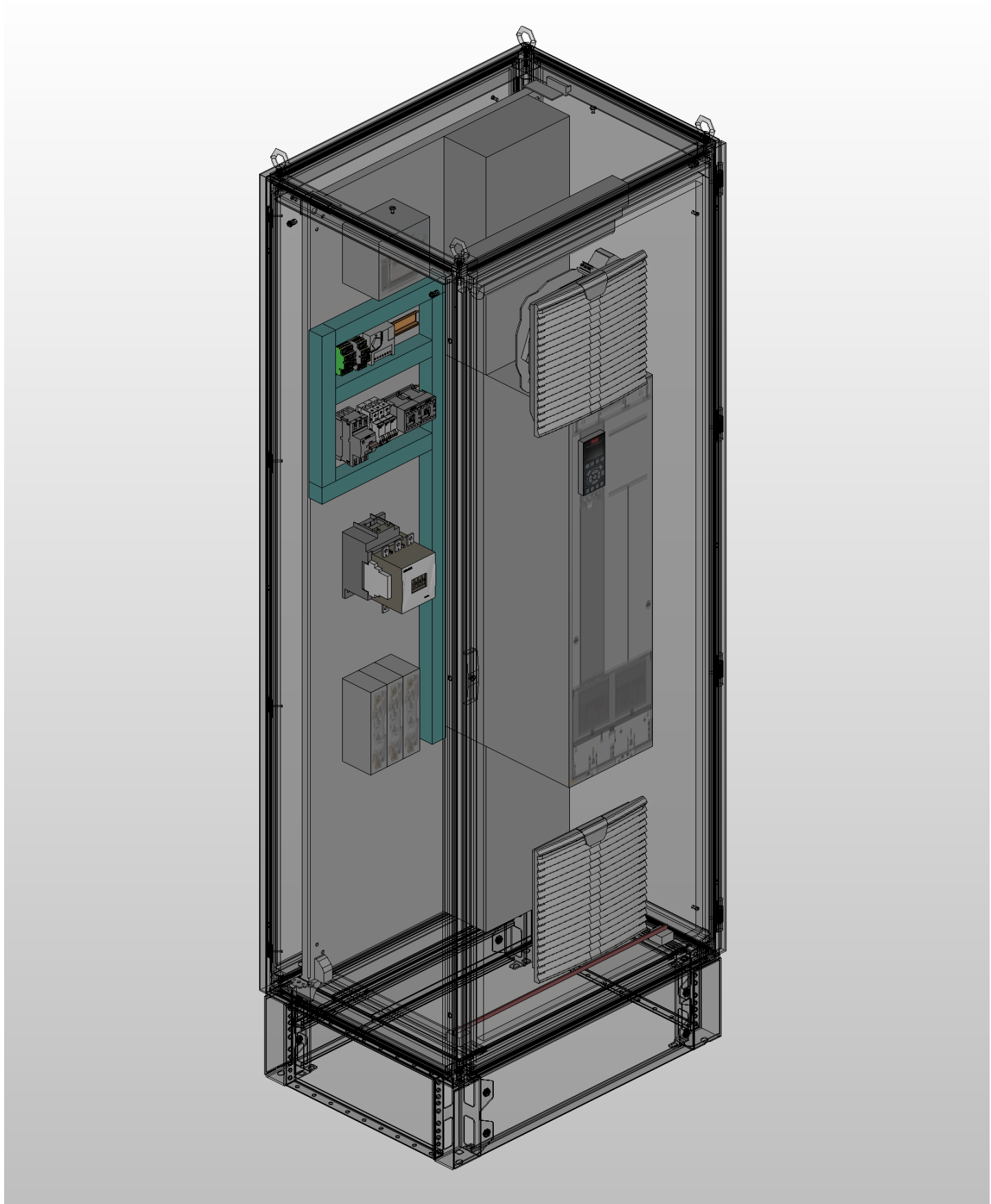
3D mounting layout 3D-Montageaufbau
