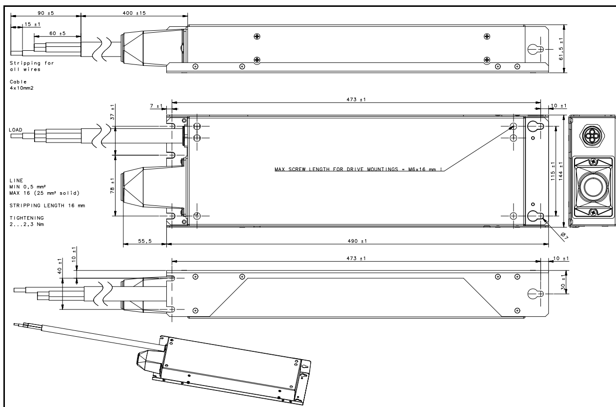
Figure 4. RFI filter assembly, size 5, dimensional drawing
