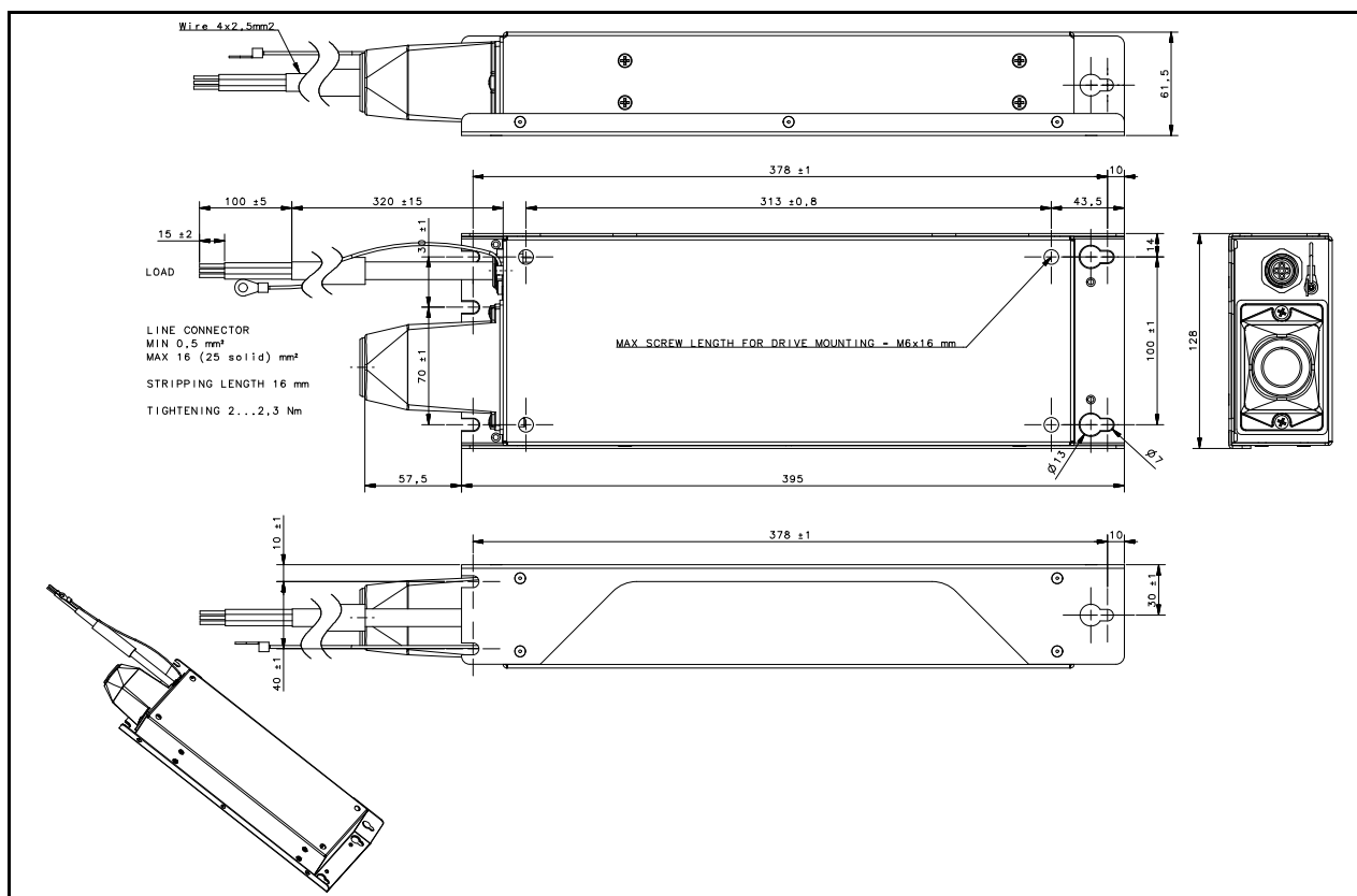
Figure 3. RFI filter assembly, size 4, dimensional drawing
